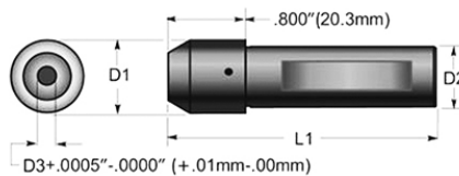
Threading Tool w/ Holder
