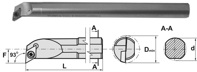
Using DCMT/DCGT Inserts
